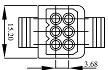
WW158B-F06E(5A/250V)
