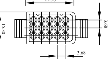
WW158B-F15E(5A/250V)
