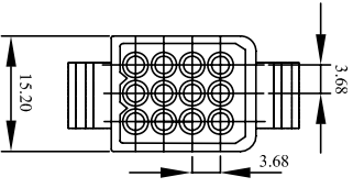
WW158B-F12-1E(5A/250V)
