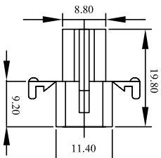
WW158B-F02E(5A/250V)
