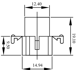
WW158B-F03E(5A/250V)
