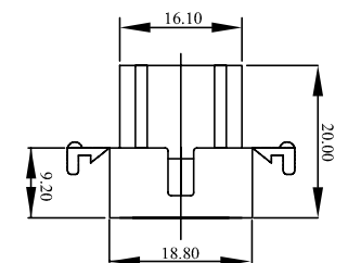
WW158B-F12-1E(5A/250V)
