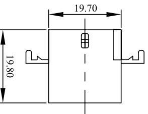
WW158B-M05E (5A/250V)
