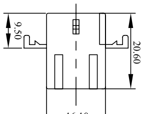
WW158B-M12E (5A/250V)
