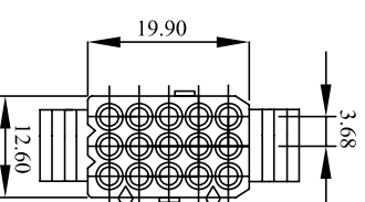
WW158B-M15E (5A/250V)
